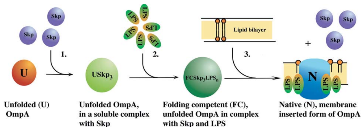
Figure 3. Scheme for an assisted folding pathway of a bacterial outer membrane protein. OmpA is translocated through the cytoplasmic membrane in an unfolded form (U) and binds to a small number of molecules of the periplasmic chaperone Skp, which solubilizes OmpA in the unfolded state (USkp 3 ). The complex of unfolded OmpA and Skp interacts with a small number of LPS molecules to form a folding-competent intermediate of OmpA (FCSkp 3 LPS n ). In the final step, folding-competent OmpA inserts and folds into the lipid bilayer (from [32]).
