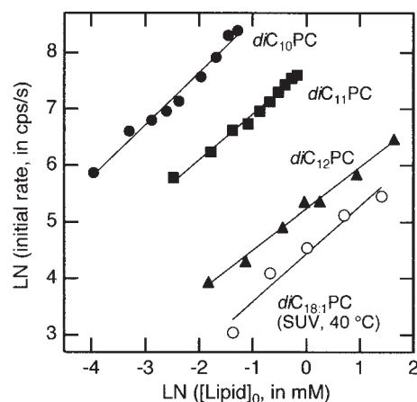
Figure 4. Double logarithmic plot of the initial rates of the OmpA folding kinetics as a function of the lipid concentrations ( T = 20^\circ\text{C} ) of the phospholipids diC 10 PC, diC 11 PC and diC 12 PC. The concentration dependence of the initial rates of OmpA folding into SUVs of diC 18:1 PC at 40 °C is shown for comparison. The data were taken from [31].
