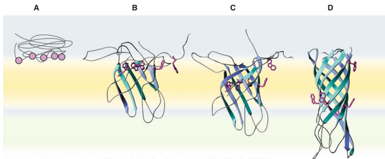
Locations of the Tryptophans of OmpA in Folding Intermediates Identified by TDFQ
