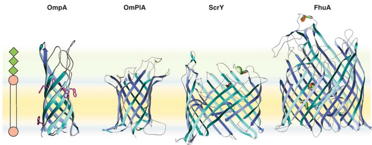
Figure 1. Some representative crystal structures of \beta -barrel membrane proteins of the outer membranes of bacteria. The different structures are characterized by TM \beta strands that span the lipid bilayer with an angle of \sim 45^\circ and often extend into the LPS region of the outer membrane. TM \beta barrels have an even number of antiparallel TM strands, which is 8 for OmpA [69], 12 for OmpA [8], 18 for ScrY [11] and 22 for FhuA [12]. OmpA is a small ion channel [29], ScrY is a sucrose-specific porin that forms trimers, FhuA is an active transporter for iron-uptake and OmpA a phospholipase that forms a dimer. Another 8-stranded TM \beta barrel is OmpX of E. coli [70]. OMPs of mitochondria are predicted to form similar TM \beta barrels. Examples are the VDAC channels, out of which more than a dozen have been sequenced [71].
