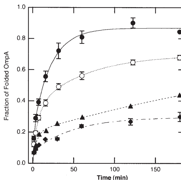
Figure 2. An assisted pathway of OmpA folding into lipid bilayers requires the simultaneous presence of Skp and LPS (data taken from Bulieris et al. [32]). Insertion and folding of OmpA were initiated by addition of preformed lipid bilayers 30 min after dilution of the denaturant urea in the absence of Skp and LPS (○); in the presence of Skp (◆); in the presence of LPS (▲) and in the presence of both Skp and LPS (●). The fractions of folded OmpA as a function of time were determined using the KTSE assay described in the text.
